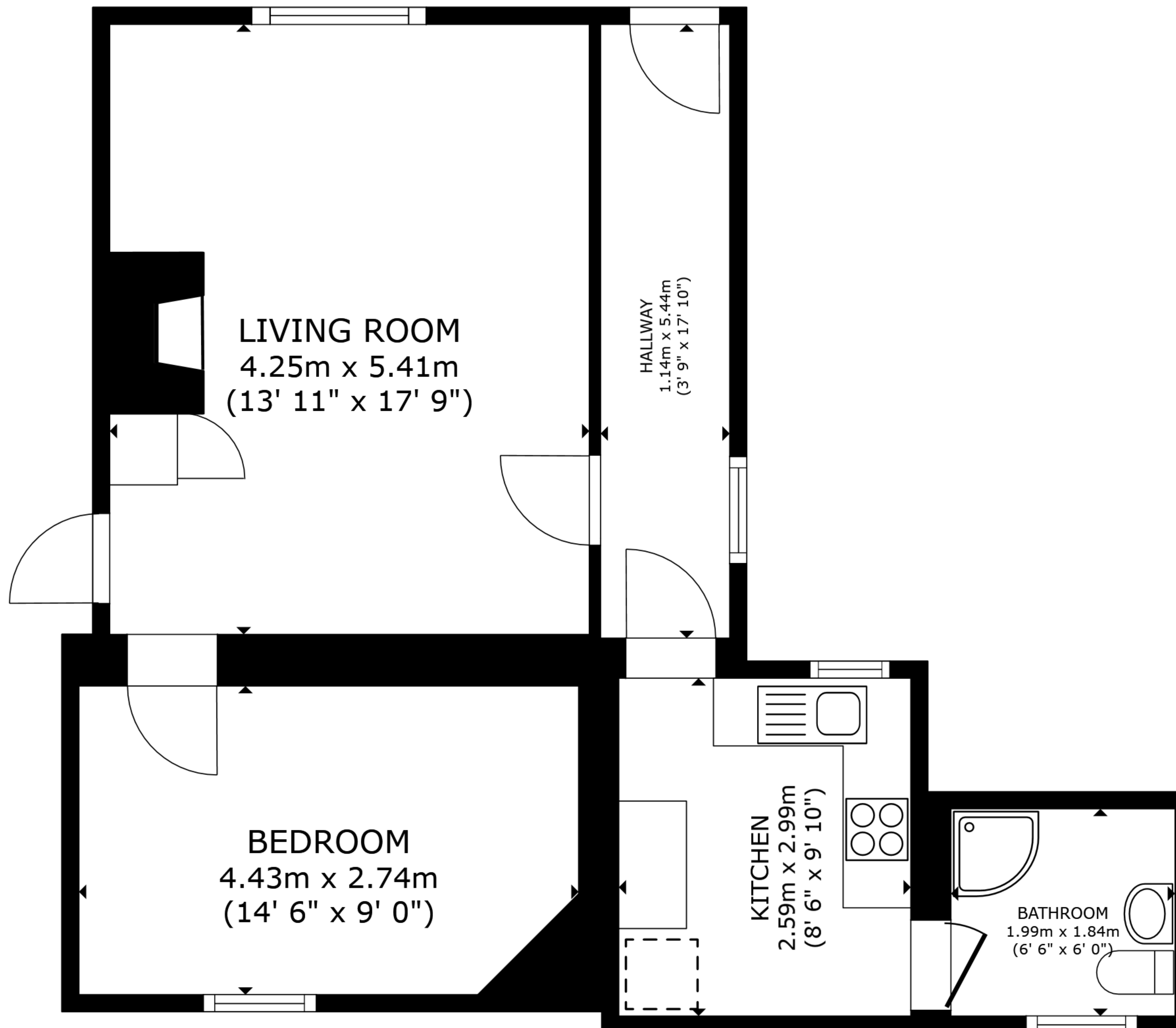
FLOOR PLAN
